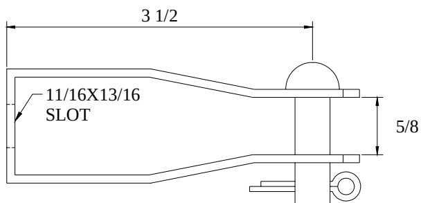
PART NUMBER A61226001
