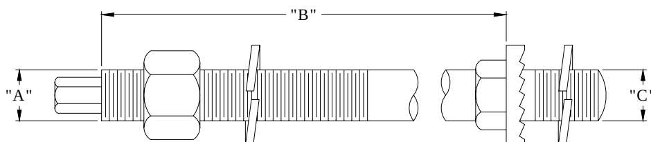
FOR STEEL ANGLE ,CHANNEL CROSSARM STAND-OFF AND POLE TOP BRACKETS PART NUMBER: 61322002
