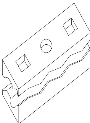
Serpentine clamp for jacketed strand Figure 8 messenger
