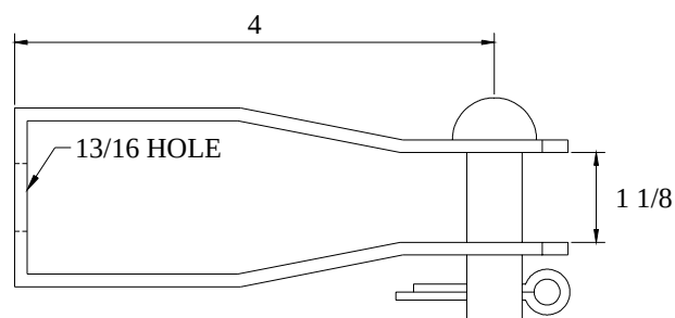
PART NUMBER A61226002
