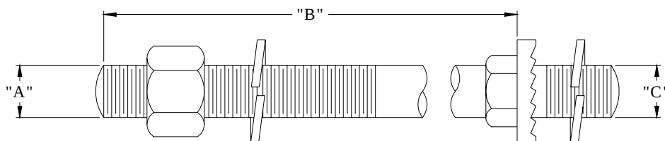
FOR STEEL ANGLE ,CHANNEL CROSSARM STAND-OFF AND POLE TOP BRACKETS PART NUMBER 61322001
