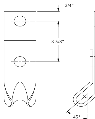
DETAIL "B"
